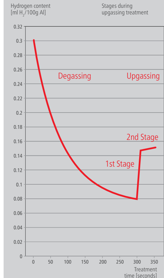
Complete treatment cycle including upgassing
